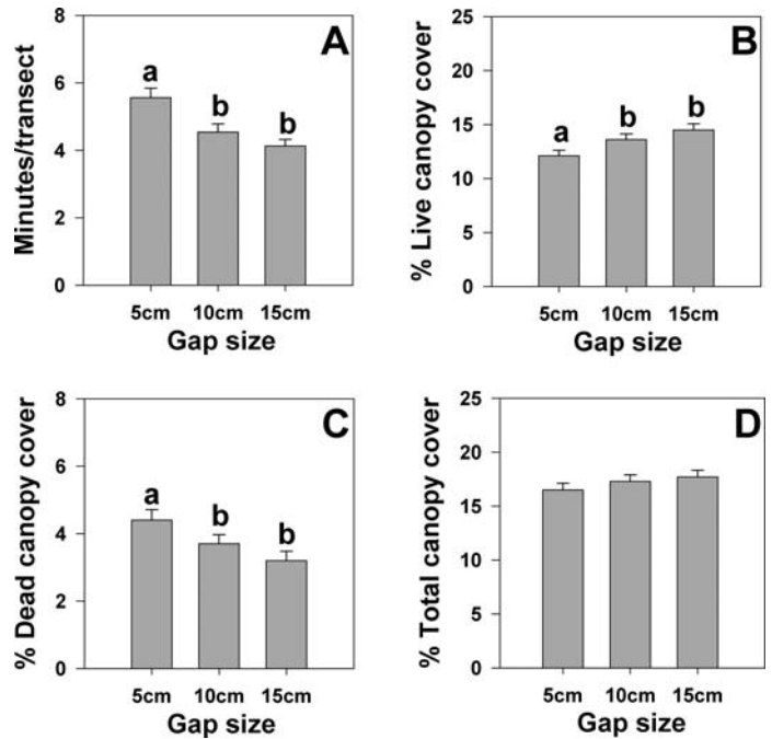
Figure 2. The effects of gap size on A , time per transect; and B , percent live; C , dead; and D , total sagebrush canopy cover for Wyoming big sagebrush communities in southeastern Oregon. Values within panels for bars without common letters are different at \alpha = 0.05 . Bars represent averages across sites and observers. Error bars are \pm 1 standard error.
